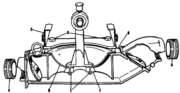
FIGURE 4 PUMP BODY AND ADJACENT PARTS
