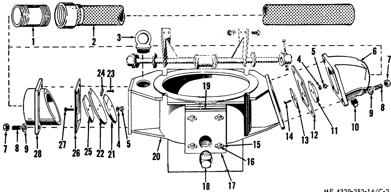
Figure No. C-2 Pump Body And Valves
