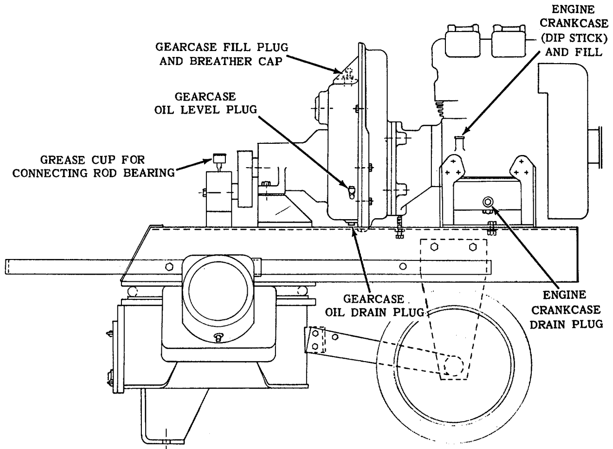
FIGURE 9 LUBRICATION CHART
